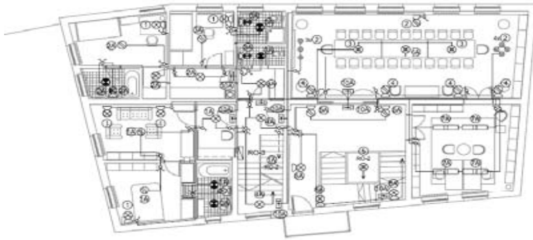
LAYOUT OF THE 1ST FLOOR - LIGHTING
